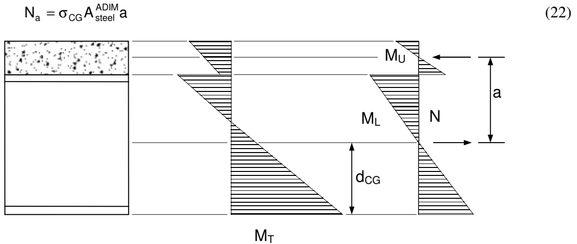
Figure 2.4. Girder - Concrete Stress Profile.
