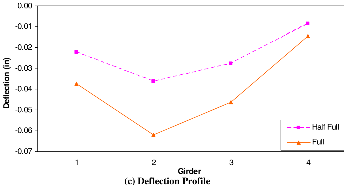
Figure 8.12. HCB Lane 2 Strains and Deflections.
