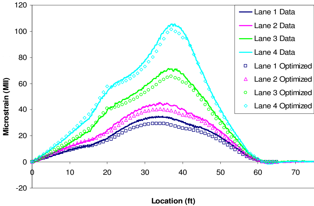
Figure 4.23. MCB Girder 5 Optimized Strain Comparison.
