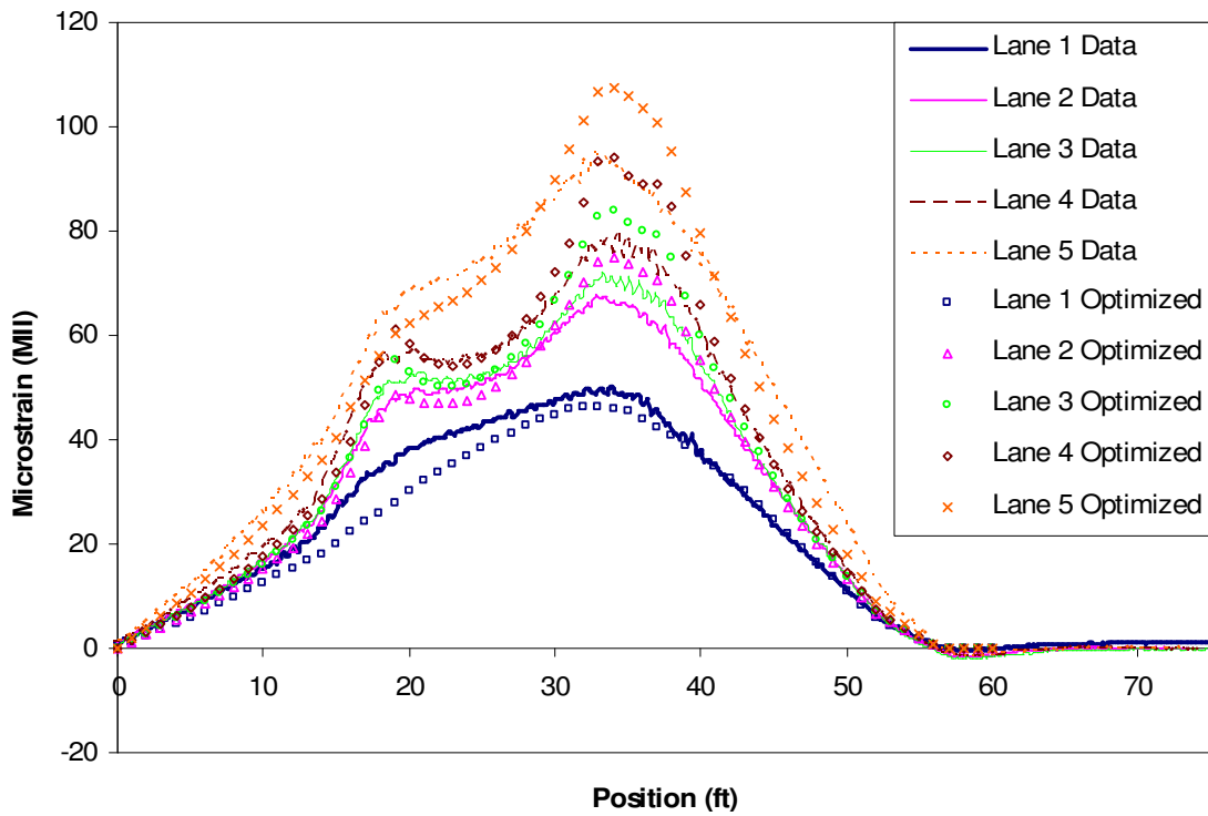
Figure 7.19. KCB2 Girder 4 Optimized Strain Comparison.
