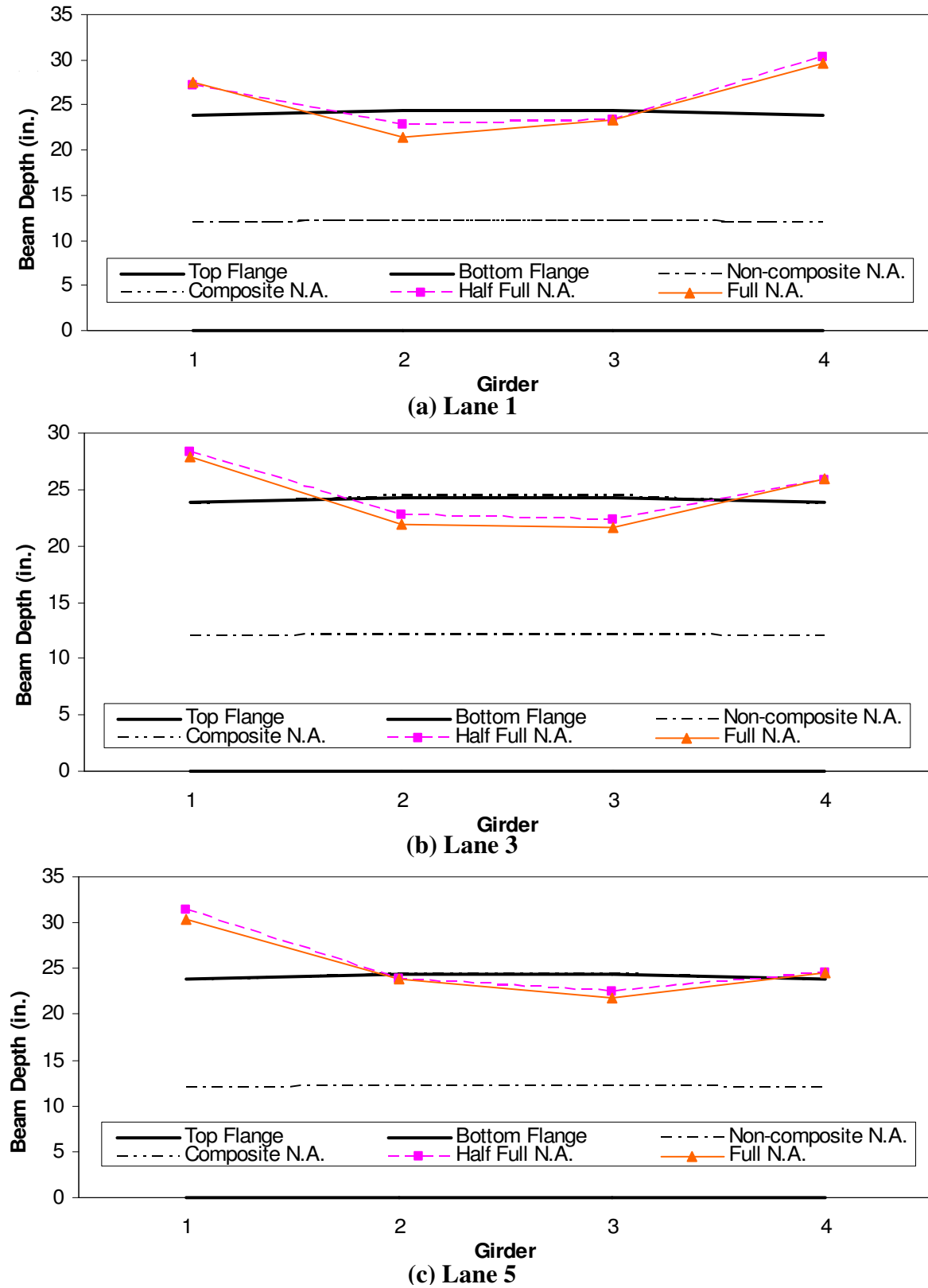
Figure 8.16.HCB Neutral Axis Locations.
